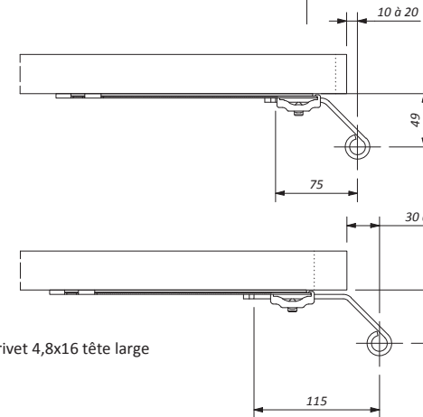
Noeud Alu Coudé 75mm
