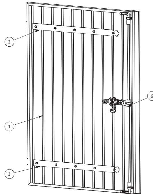
VB - Penture contre-penture
