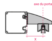
Poteau 188x188
