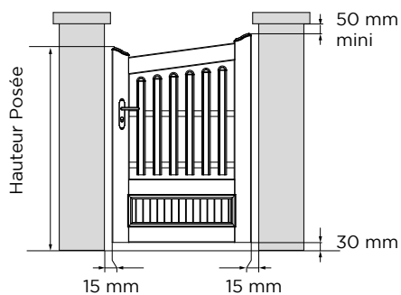
PORTILLON
