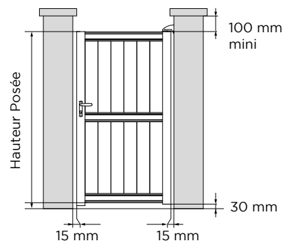
PORTILLON
