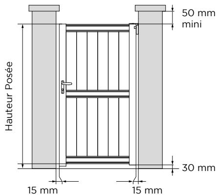
PORTILLON
