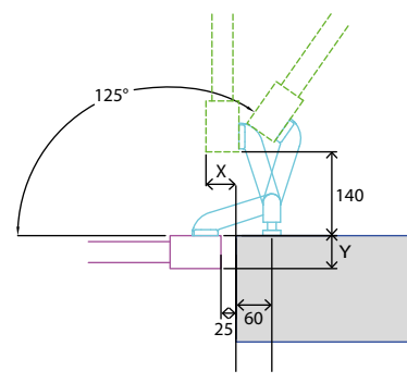
Pentures 180°
