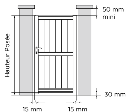
PORTILLON
