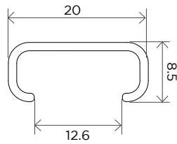
Clip finition
